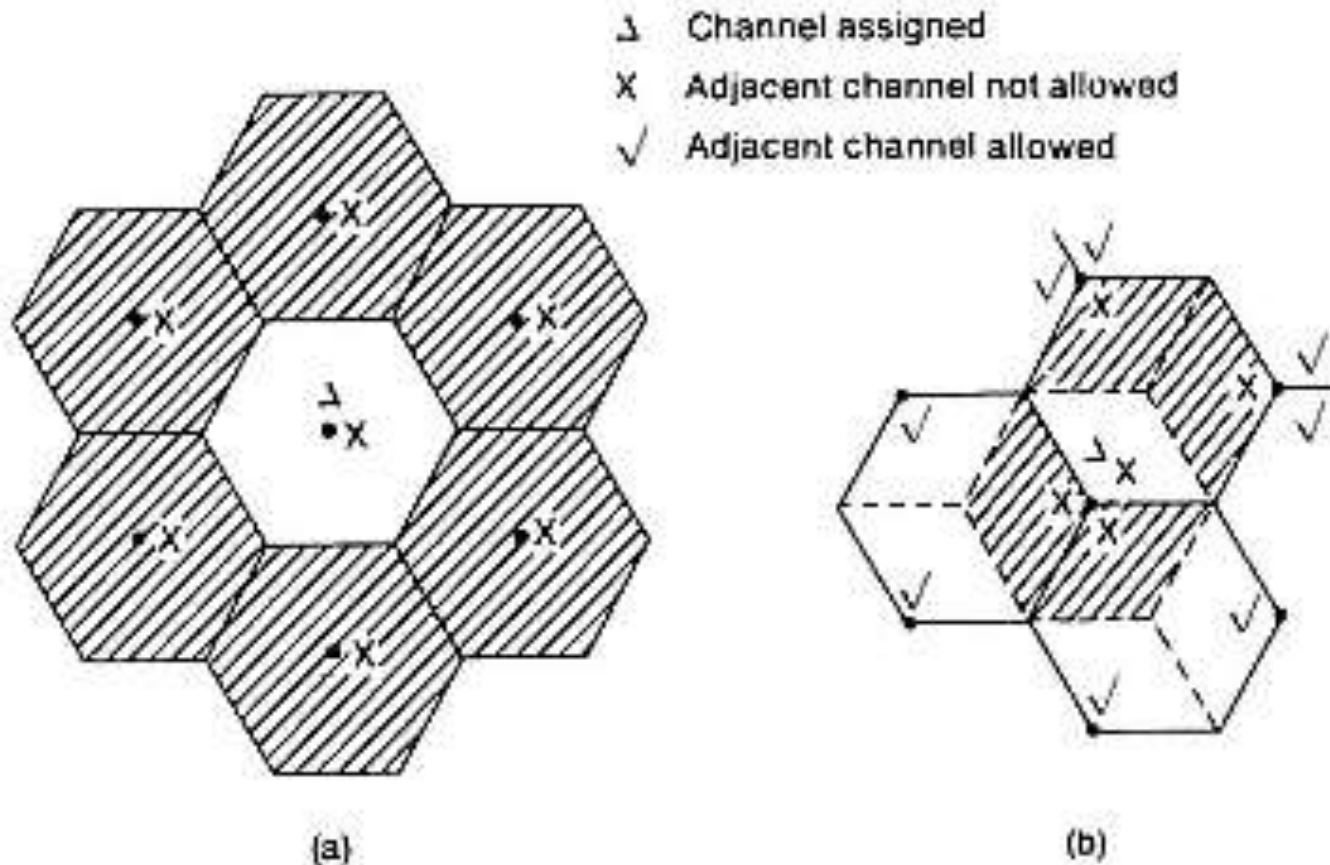
Adjacent channel assignment. (a) Omnidirectional-antenna cells (b) directional-antenna cells
