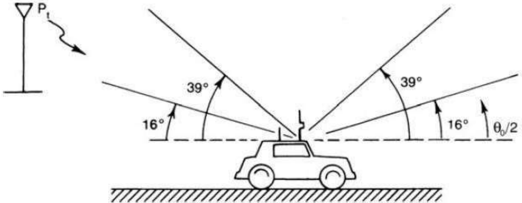
FIGURE 8.49 Vertical angle of signal arrival.
